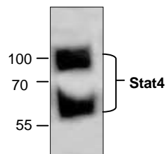
Cat.#: 3471R-100 Western blot analysis of Stat4 expression in rat kidney tissue lysate.
