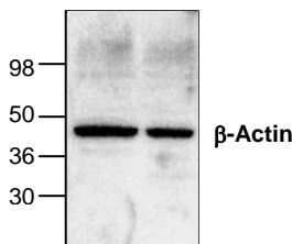
Cat.# 3662-100 Western blot analysis of \beta -Actin in Jurkat cell lysate (left lane) and mouse intestine tissue lysate (right lane).
