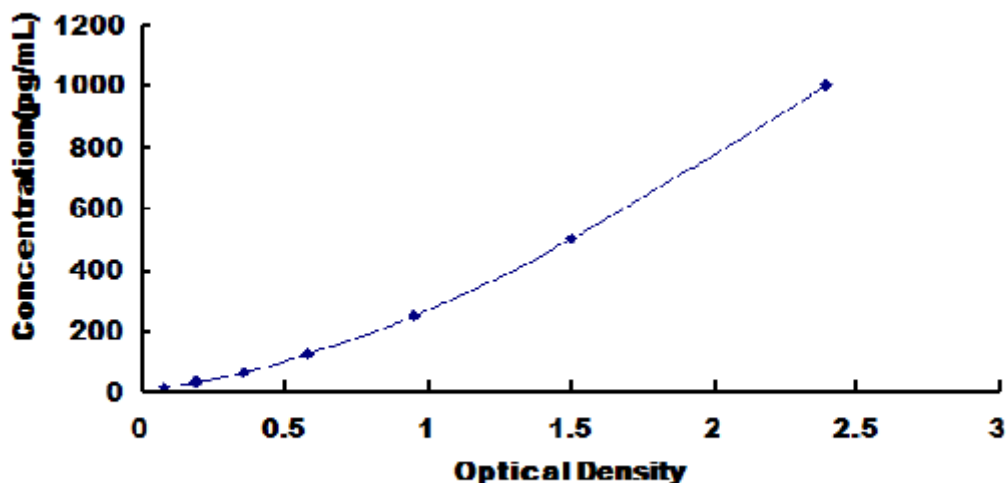
Typical Standard Curve for Mouse IL6 ELISA.
