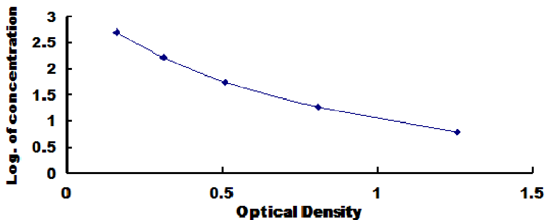
Typical Standard Curve for CORT ELISA.
