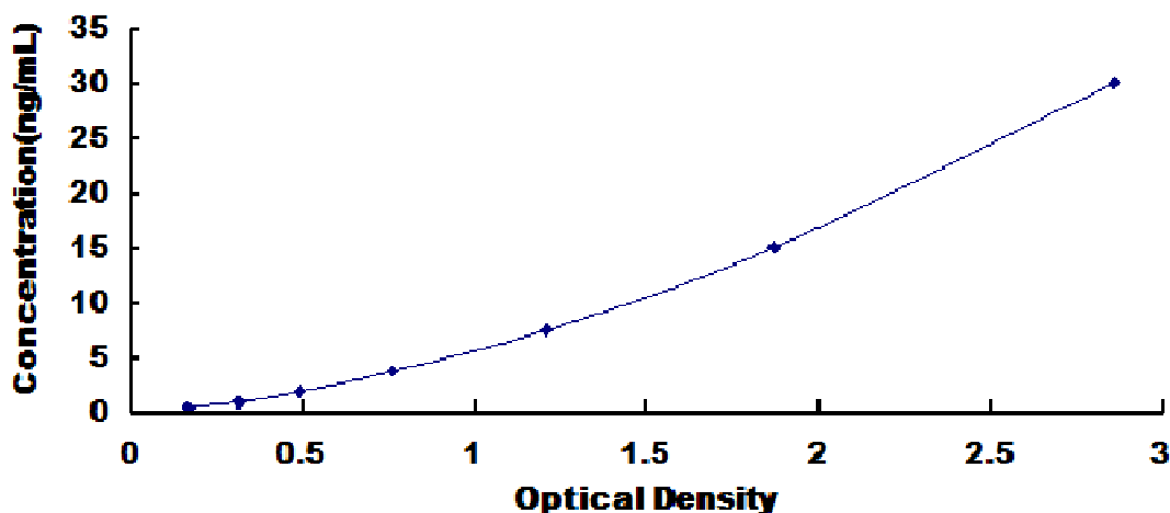
Typical Standard Curve for Human ELN ELISA.
