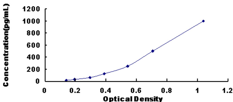
Figure 1: Typical Standard Curve for Mouse IL20 ELISA.
